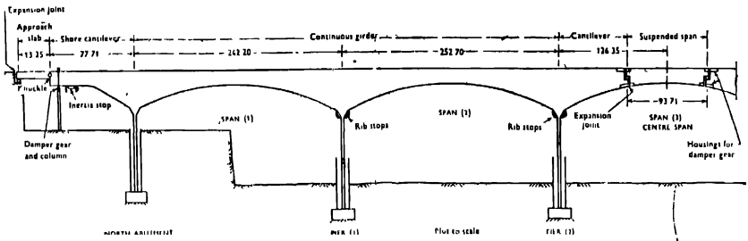
Fig. 352.—Waterloo Bridge, London : Articulation Diagram (see previous page).
